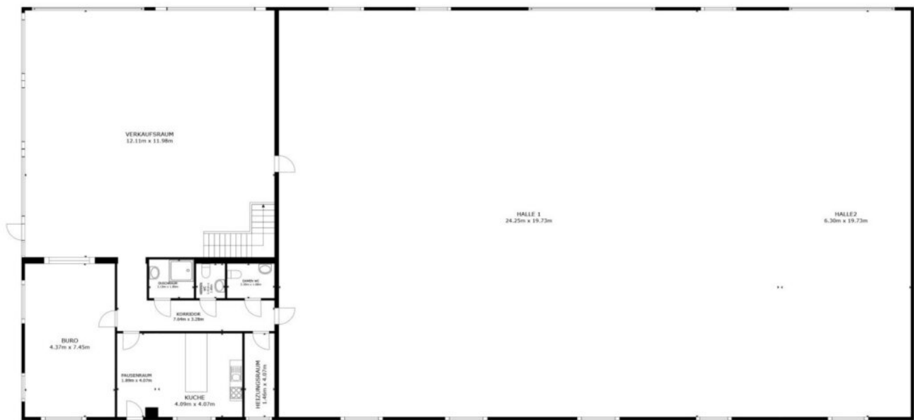
FLOOR 1
