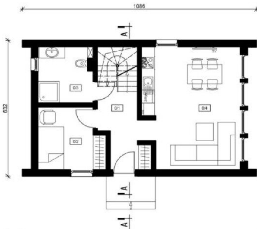
1st FLOOR, 1:150
