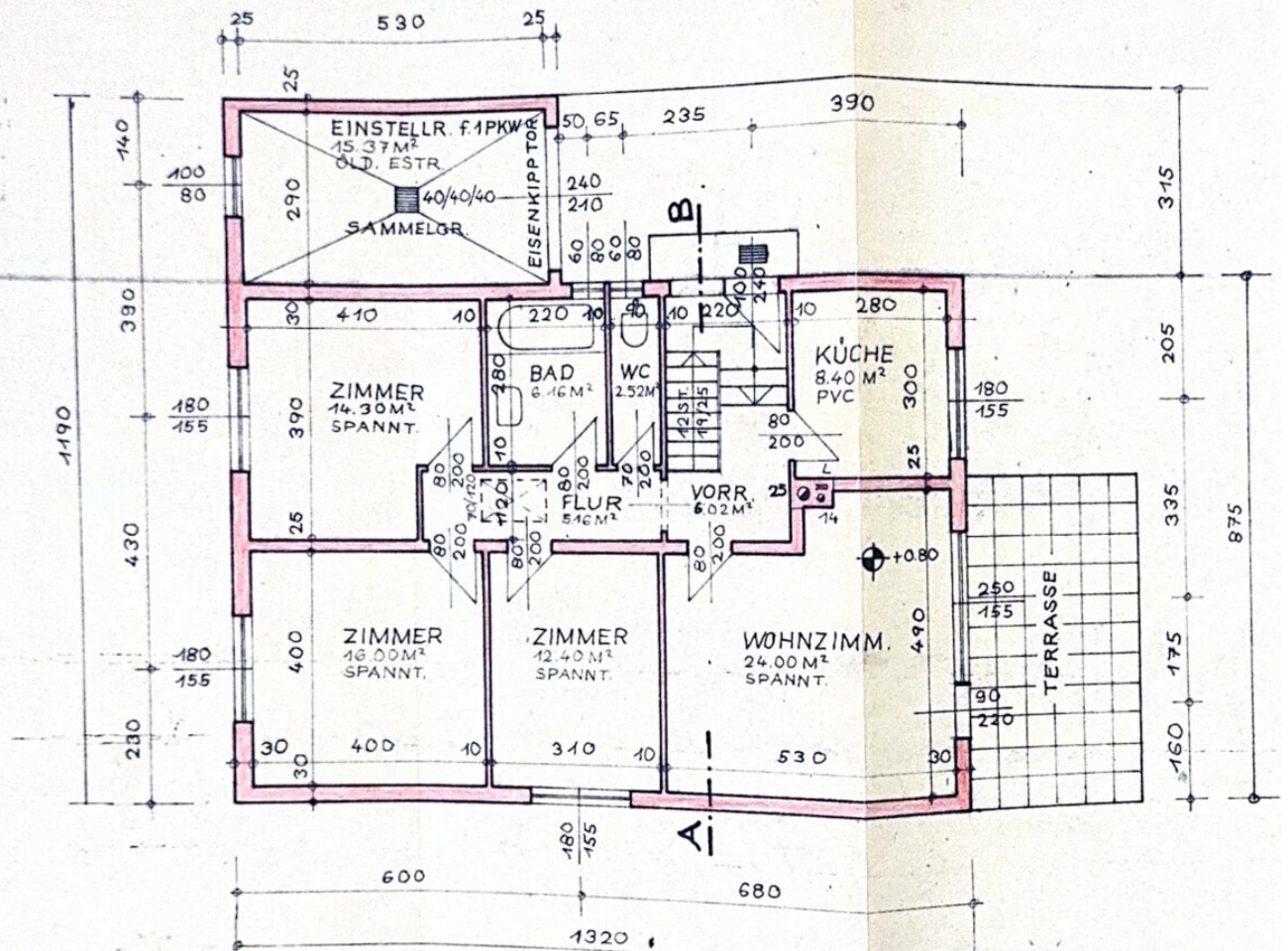
ERDGESCHOSS M = 1:100
