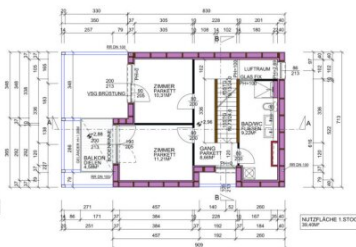
GRUNDRISS 1. STOCK
