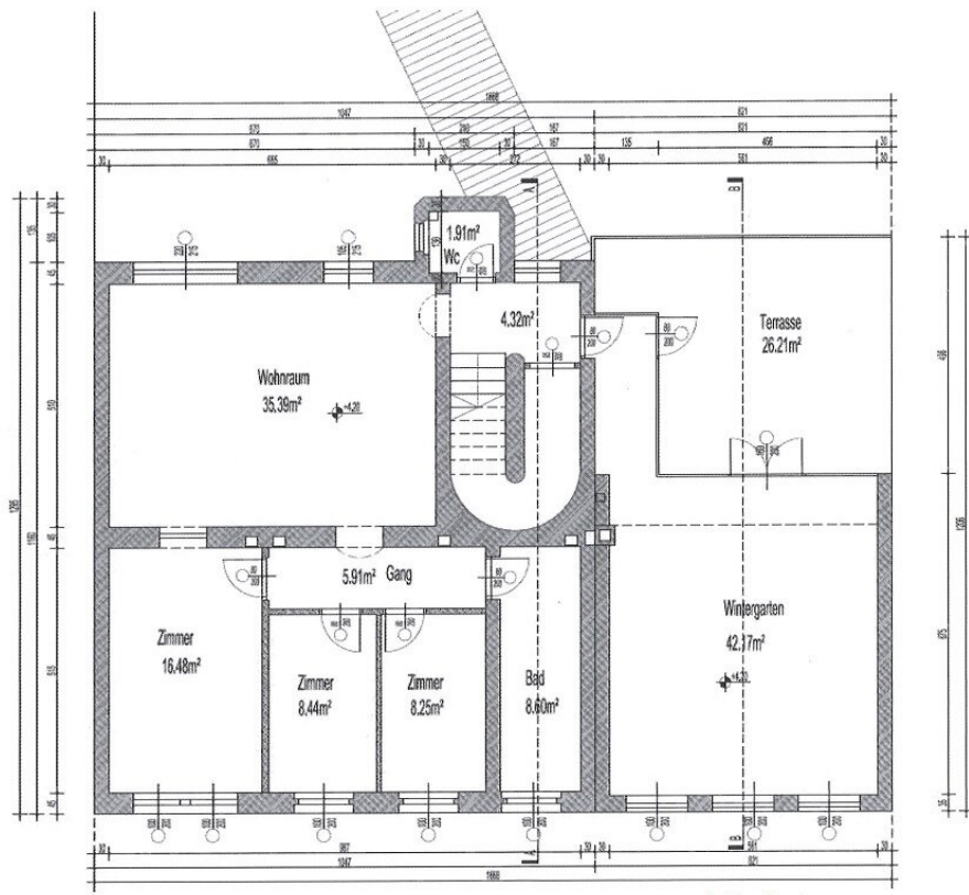
1. Stock
