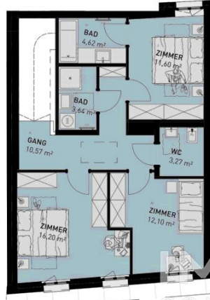
+1 OBERGESCHOSS
