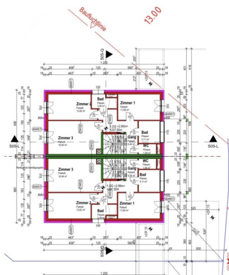
Ebene +1 (Obergeschoss)
