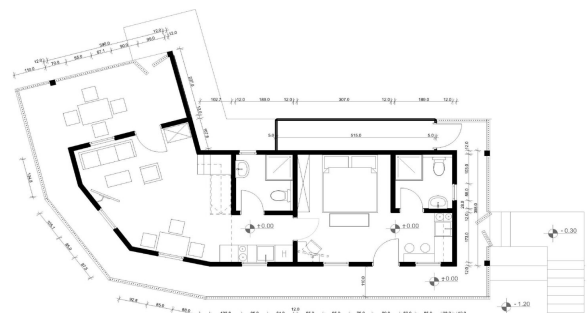
Grundriss Apartment 1 + 2
