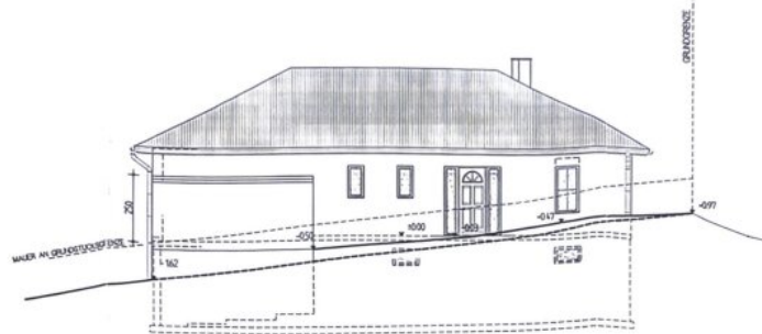
ANSICHT NORTHWEST
