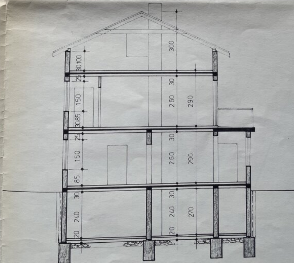
S C H N I T T A - B
