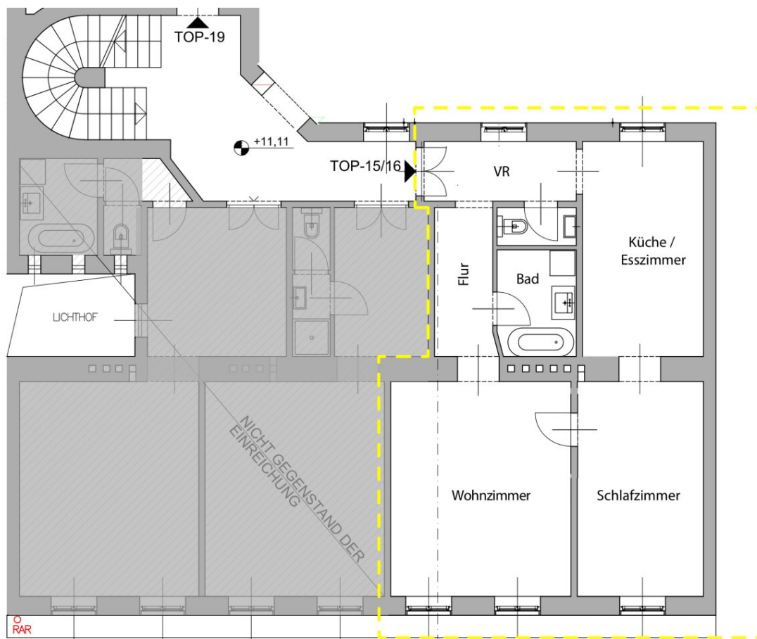
Grundriss 3.Stock
