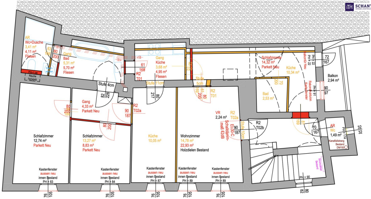
GRUNDRISS 3. STOCK | M = 1:100
