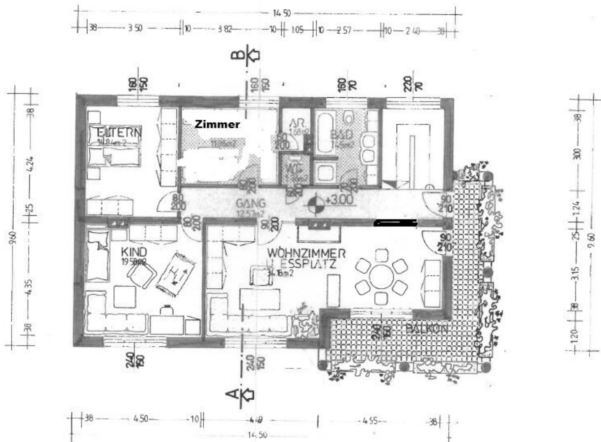
GRUNDRISS - 1. STOCK 102.64 m 2
