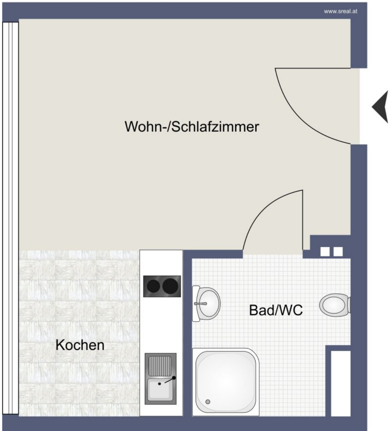
Skizze 2. Stock
