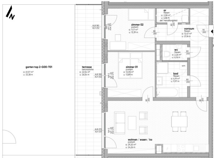
grundriss M 1: 75
